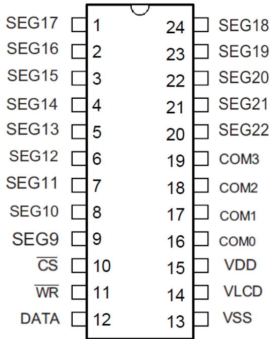
HT1621BD SSOP 24
