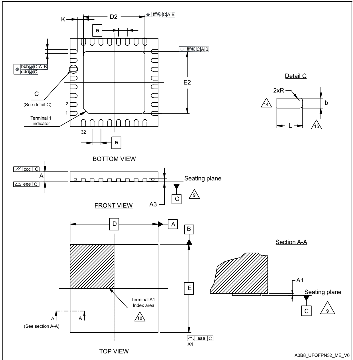
Figure 40. UFQFPN32 - Outline
