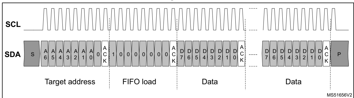
Figure 25. FIFO load
