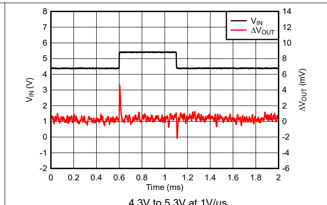
Figure 7-11. TPS76933 Line Transient Response (New Chip)
