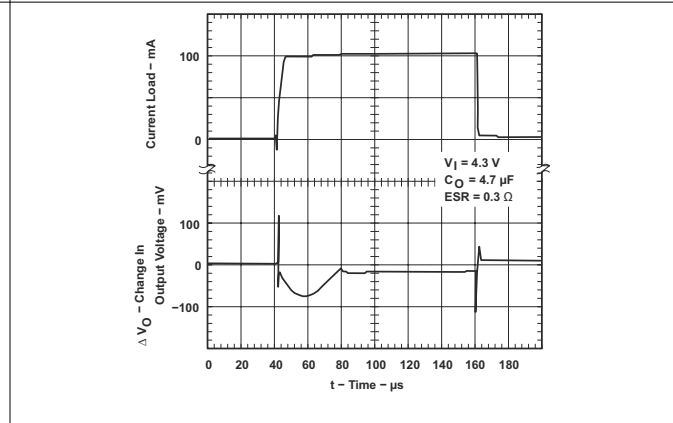
Figure 7-13. TPS76933 Load Transient Response (Legacy Chip)
