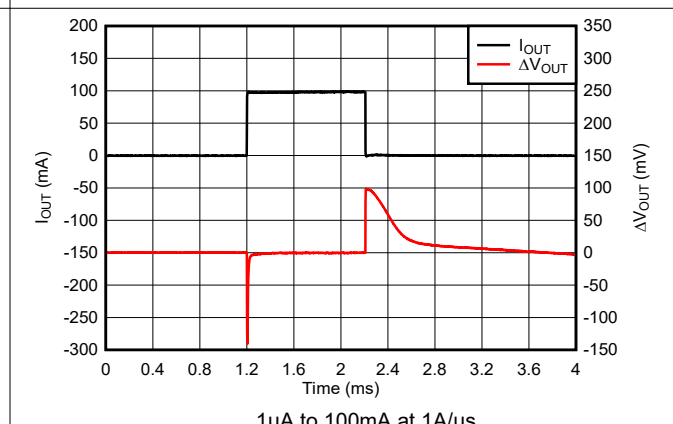
Figure 7-15. TPS76933 Load Transient Response (New Chip)
