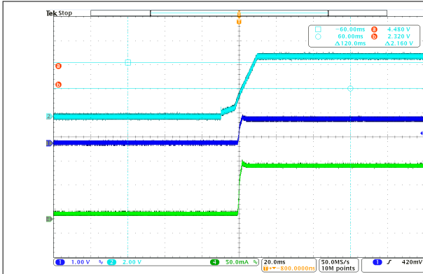
Channel 1 = V_{OUT} , channel 2 = V_{IN} , channel 4 = I_{OUT} Figure 7-4. Power-Up Waveform (Legacy Chip)
